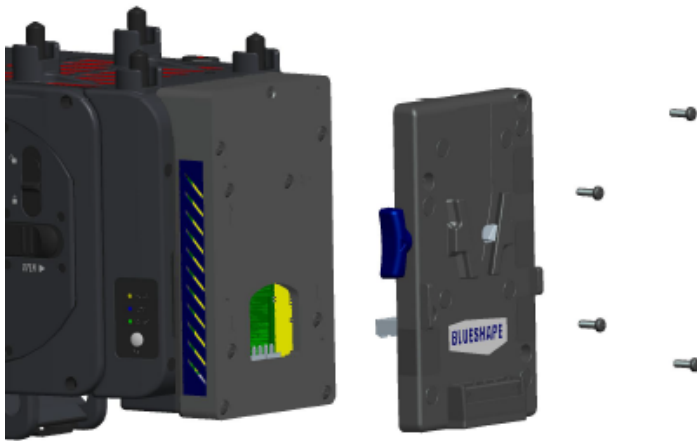
3. Connect the 6 pole connector to the adapter main board through the large hole in the back; Fix the V-Plate on the adapter body with the 4 x 14mm screws provided
