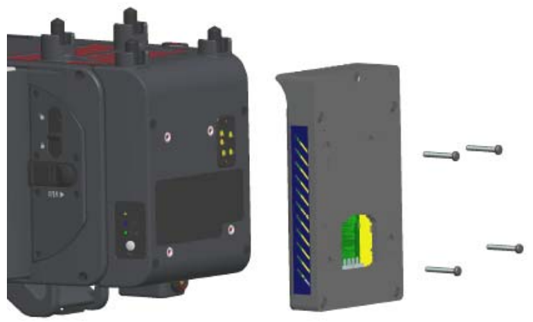
2. Fixing the adapter using 4 x 23mm screws
